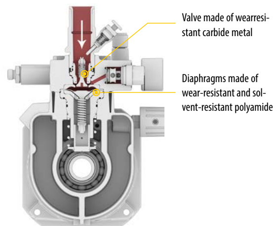
Fig.: This geometry allows the diaphragms to move smoothly, ensuring both reliability and durability.
